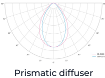
Prismatic diffuser
